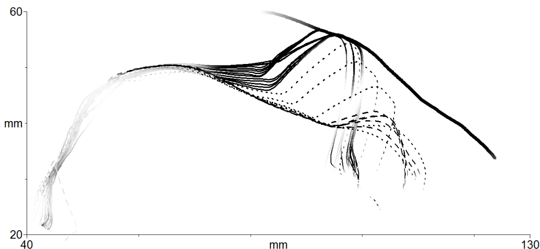
Figure 5. Tongue surface contours of successive frames throughout the production and release of a click. 306Hz sample rate. Solid lines= pre-release rarefaction; Dotted = release phase; Dashed lines = recoil from floor of mouth. Faded contours show low confidence of auto-fit.
